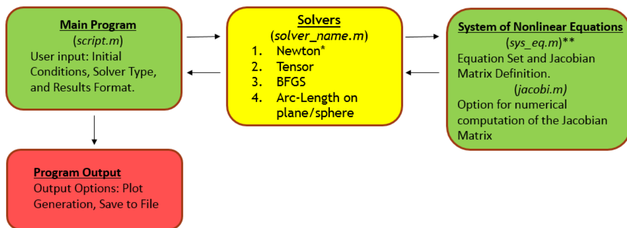
Figure 4. Program flowchart
