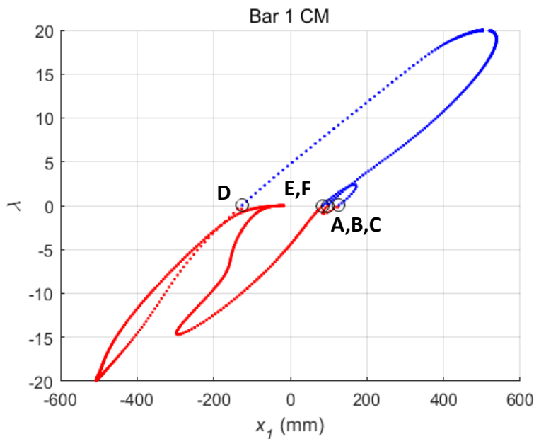
Figure 24. Total solution curve for bar one x position, k_s = 87.6 N/m
